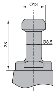
Type: G BT 35 pull stud Heian, Shoda
